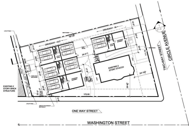
Proposed Lower Level Site Plan Parking / Drive
